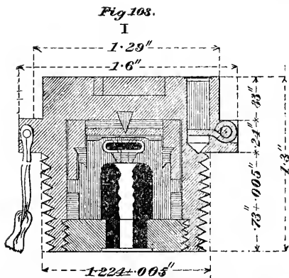
Royal laouratory percussion fuzes I and II.
